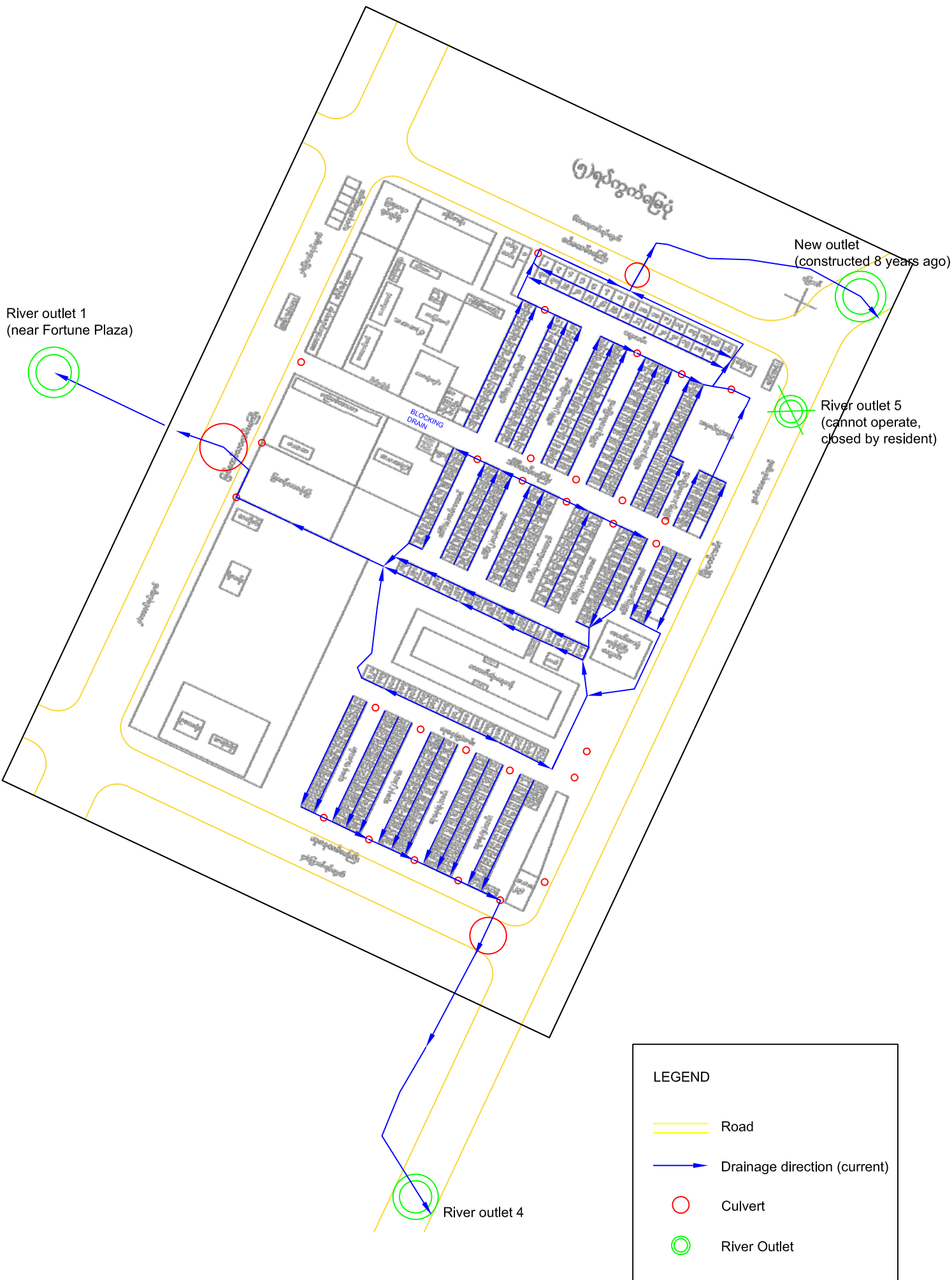
Current drainage system of Ward 5 Thaketa
